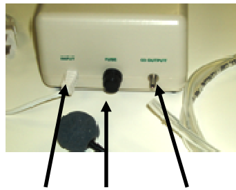
Power Cord Fuse holder Hose output connector
